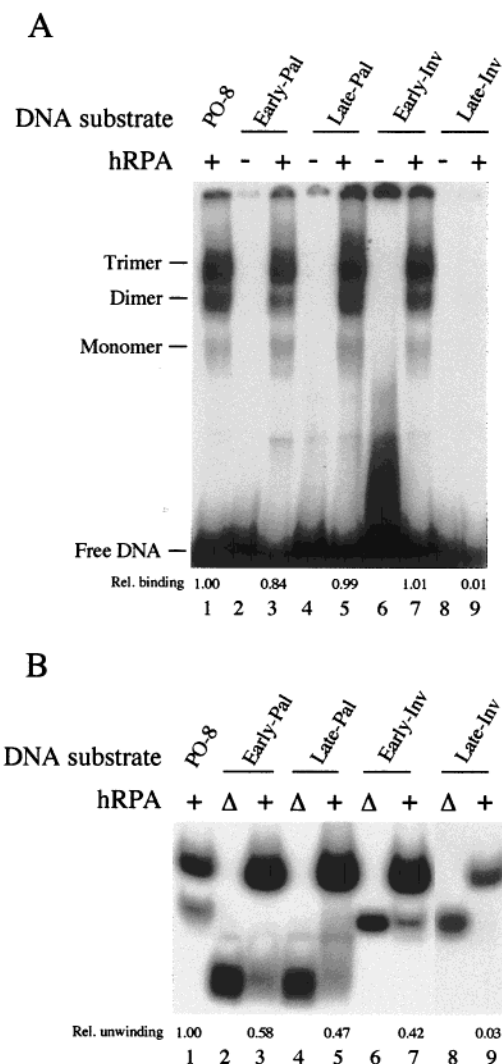
FIGURE 6: Effect of the duplex flank sequence on pseudo-origin binding and unwinding by hRPA. Each pseudo-origin substrate (0.15 pmol; 5'- 32 P-labeled), as indicated (shown in Figure 5), was incubated with or without 1.5 pmol of hRPA under standard binding (A) and unwinding (B) reaction conditions. The reaction products were then separated by native gel electrophoresis and visualized by autoradiography. The identity of the generated ssDNA was established by comparison with the top strand of each substrate (Δ). The locations of hRPA–DNA complexes, the unbound PO substrate, and the duplex and single-stranded DNA forms of the substrates are shown. The level of substrate binding and unwinding was quantified as described in the legend of Figure 2.
